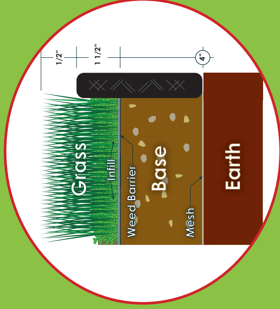
Cutaway view of the finished install.
